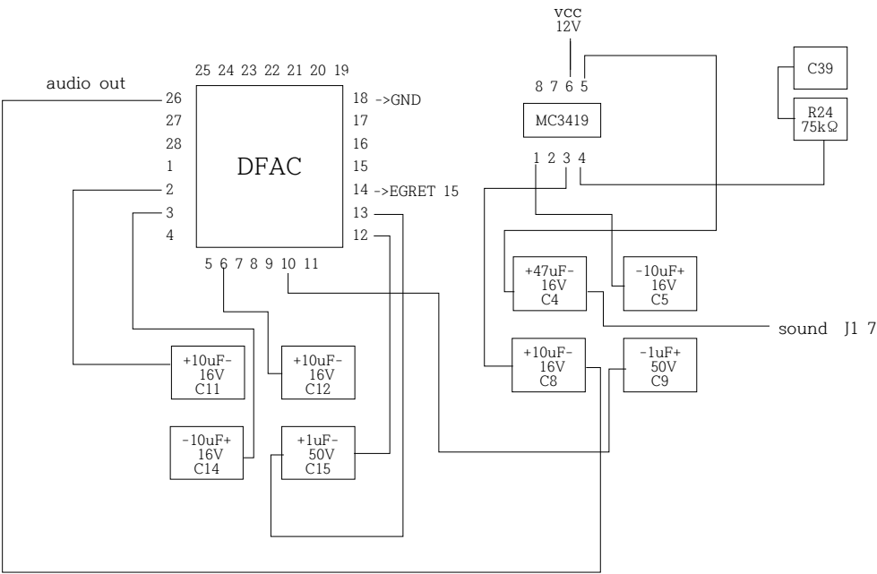
MC3419 (audio amp chip)
